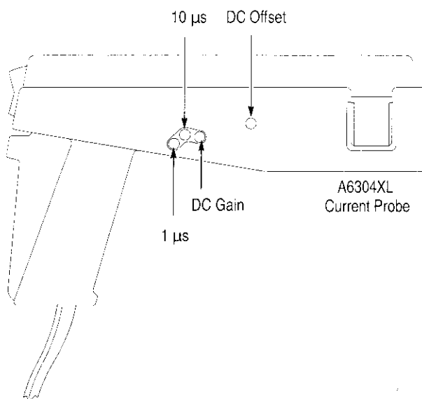
Figure 6–6: A6304XL Adjustment Locations
