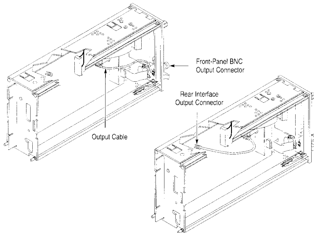
Figure 7-8: Using the Rear Interface Output Connector
