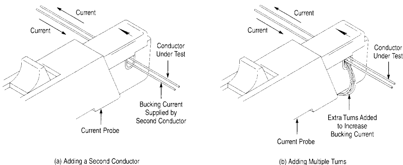
Figure 3-4: Increasing the DC Measurement Range
