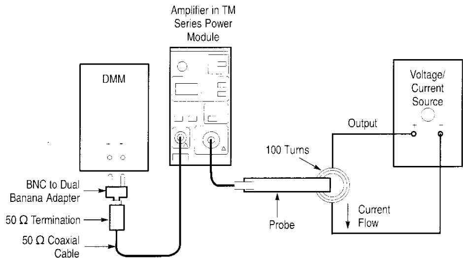
Figure 5-4: DC Accuracy Test Setup for A6302/A6302XL: 100 mA to 5 A
