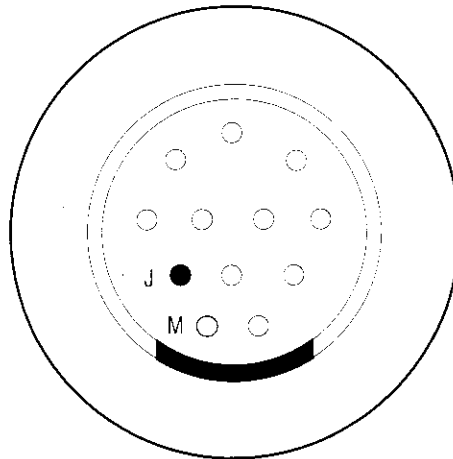
Figure 6–4: Current Probe Connector Configuration
